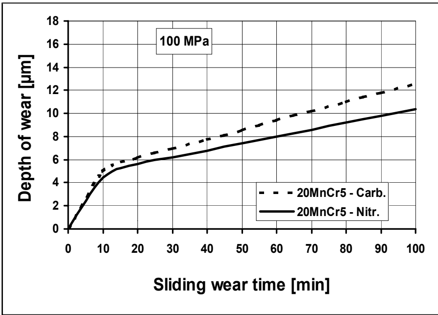
Comparison of wear resistance under two levels of unit load of 20MnCr5 steel, carburized and nitrated in controlled process
