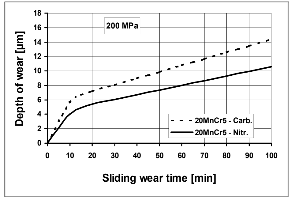
Comparison of wear resistance under two levels of unit load of 20MnCr5 steel, carburized and nitrated in controlled process
